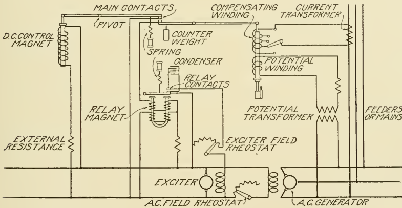
Fig. 19. Diagram of Tirrill Regulator Operating on Field of Exciter
